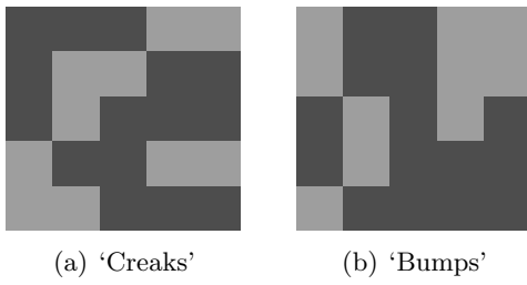
Figure 23.6: Localising the burglar. The latent variable h_t \in \{1, \dots, 25\} denotes the positions, defined over the 5 \times 5 grid of the ground floor of the house. (a) : A representation of the probability that the ‘floor will creak’ at each of the 25 positions, p(v^{creak}|h) . Light squares represent probability 0.9 and dark square 0.1. (b) : A representation of the probability p(v^{bump}|h) that the burglar will bump into something in each of the 25 positions.
