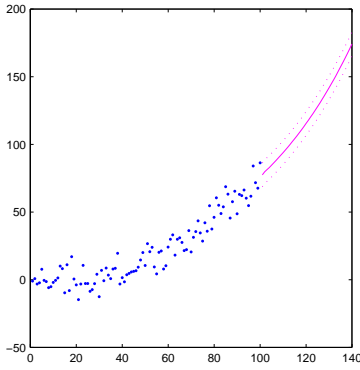
Figure 24.1: Fitting an order 3 AR model to the training points. The x axis represents time, and the y axis the value of the timeseries. The solid line is the mean prediction and the dashed lines \pm one standard deviation. See demoARtrain.m
