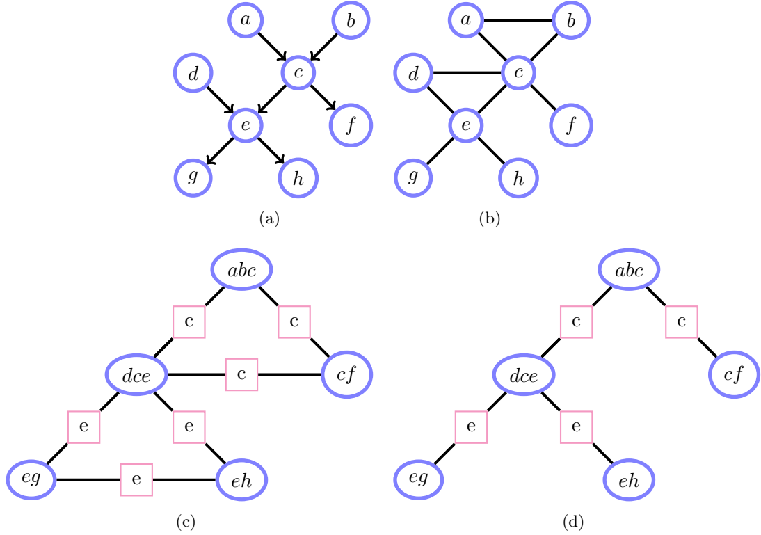
Figure 6.4: (a) : Belief Network. (b) : Moralised version of (a). (c) : Clique Graph of (b). (d) : A junction tree. This satisfies the running intersection property that for any two nodes which contain a variable in common, any clique on the path linking the two nodes also contains that variable.
