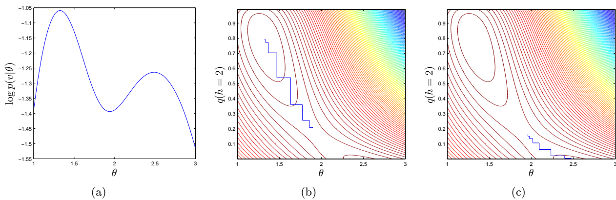
Figure 11.2: (a) : The log likelihood for the model described in example(51). (b) : Contours of the lower bound LB(q(h = 2), \theta) . For an initial choice q(h = 2) = 0.5 and \theta = 1.9 , successive updates of the E (vertical) and M (horizontal) steps are plotted. (c) : Starting at \theta = 1.95 , the EM algorithm converges to a local optimum.
