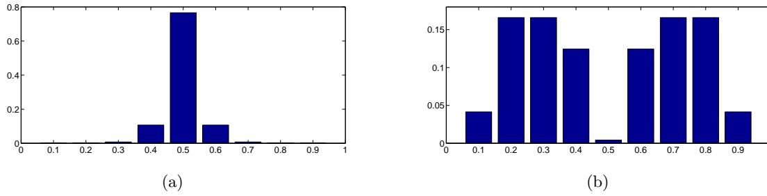
Figure 12.1: (a) : Discrete prior model of a ‘fair’ coin. (b) : Prior for a biased ‘unfair’ coin. In both cases we are making explicit choices here about what we consider to be a ‘fair’ and an ‘unfair’.
