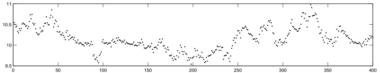
Figure 25.11: Data from an intermittent mean-reverting process. See exercise(240).
