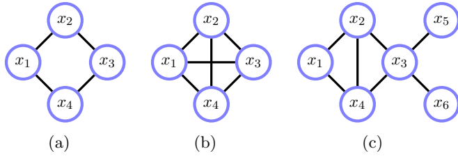
Figure 4.1: (a): p_a = \frac{\phi(x_1, x_2)\phi(x_2, x_3)\phi(x_3, x_4)\phi(x_4, x_1)}{Z_a} . (b): p_b = \frac{\phi(x_1, x_2, x_3, x_4)}{Z_b} . (c): p_c = \frac{\phi(x_1, x_2, x_4)\phi(x_2, x_3, x_4)\phi(x_3, x_5)\phi(x_3, x_6)}{Z_c} .
