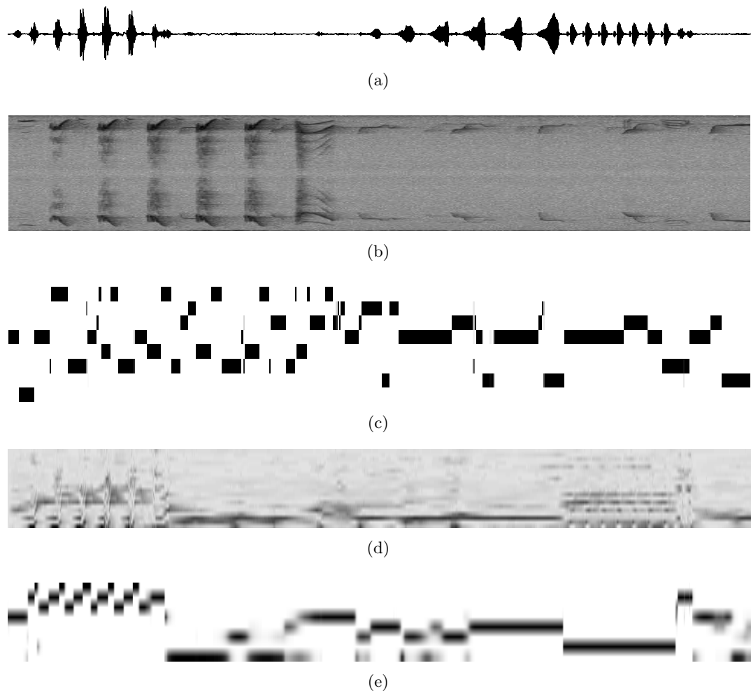
Figure 24.3: (a) : The raw recording of 5 seconds of a nightingale song (with additional background birdsong). (b) : Spectrogram of (a) up to 20,000 Hz. (c) : Clustering of the results in panel (b) using an 8 component Gaussian mixture model. The index (from 1 to 8) of the component most probably responsible for the observation is indicated vertically in black. (d) : The 20 AR coefficients learned using \sigma_v^2 = 0.001 , \sigma_h^2 = 0.001 , see ARlds.m . (e) : Clustering the results in panel (d) using a Gaussian mixture model with 8 components. The AR components group roughly according to the different song regimes.
