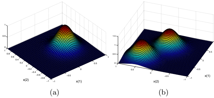
Figure 17.8: (a): The output of an RBF function \exp(-\frac{1}{2}(\mathbf{x} - \mathbf{m}^1)^2/\alpha^2) . Here \mathbf{m}^1 = (0, 0.3)^T and \alpha = 0.25 . (b): The combined output for two RBFs with \mathbf{m}^1 as above and \mathbf{m}^2 = (0.5, -0.5)^T .
